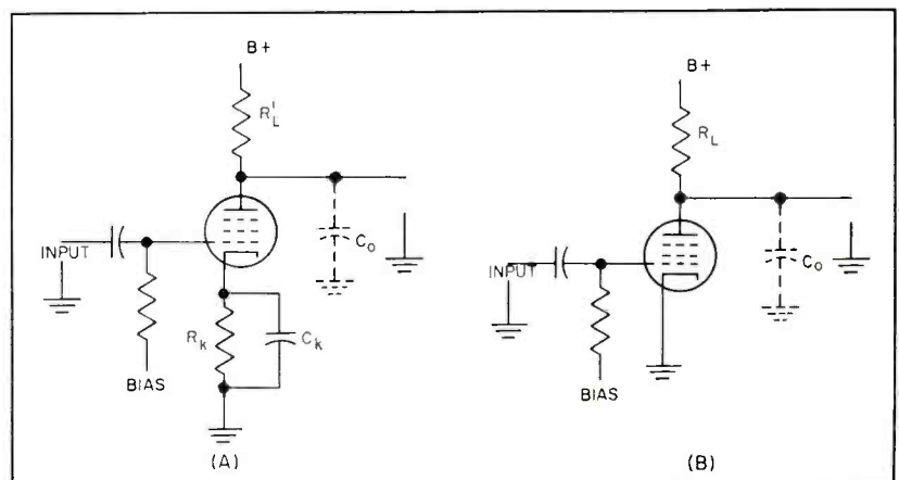
FIG. 5—Cathode-compensated amplifier stage (A) and conventional stage (B)
