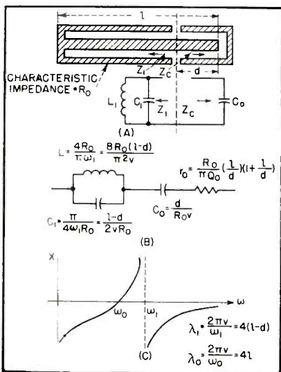
FIG. 3—Basic physical form for resonant leg of bridge (A) with equivalent circuit (B) and reactance-versus-frequency plot (C)
