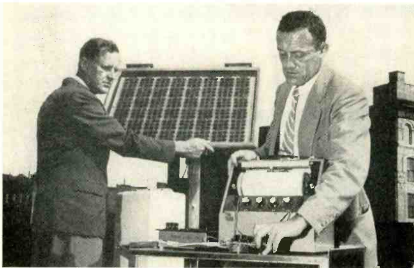
SOLAR battery developed by Bell Laboratories gets final tests before shipment.
