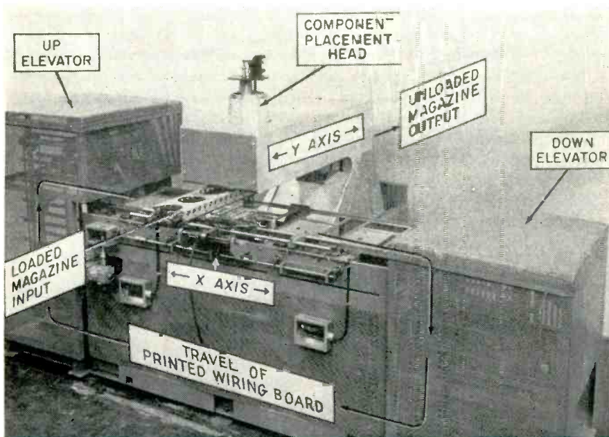
ASSEMBLY MACHINE —Servo-positioned insertion head (right) fits into center of elevator and conveyor mechanism that recycles 20 wiring boards under head until all required components have been inserted one by one. Elevators also provide required storage space at each end to accommodate adjacent machines having different operating times.
