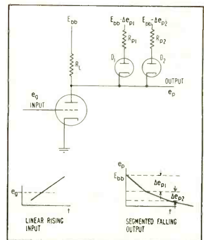
FIG. 1—Nonlinear function generator uses biased diodes to shape waveform
