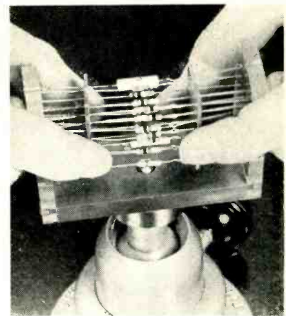
Pushing boards together after installation of components
