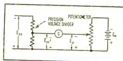
FIG. 3—Potentiometer circuit for measuring sawtooth voltage level
