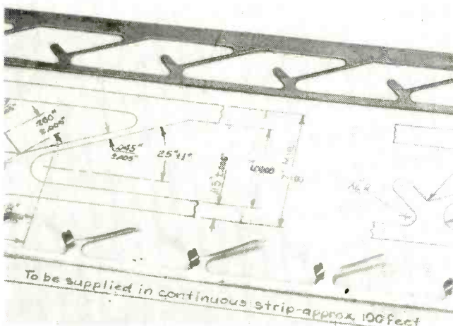
FIG. 3—Filament bus strips as blanked (top) and trimmed for use
