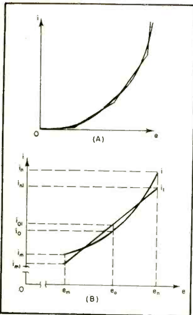
FIG. 1—Square-law characteristic showing segmented approximation (A) and isolated segment (B)
