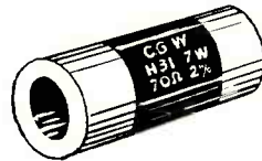
HIGH-FREQUENCY—STYLE H • Combine high-power with excellent high-frequency characteristics. Resistance film is continuous, spiraled or striped according to resistance range or application. Silver metallized bands fired-on ends for termination. Silicone coated: water-cooled types uncoated.
