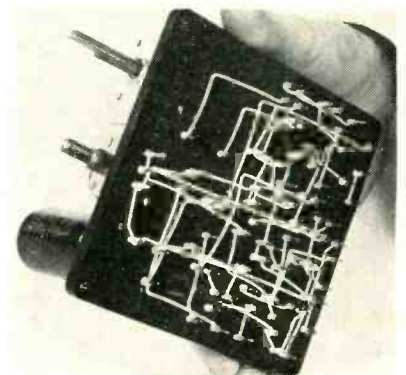
Bottom view of plastic panel for five-tube radio, showing solderless wiring put on by machine
