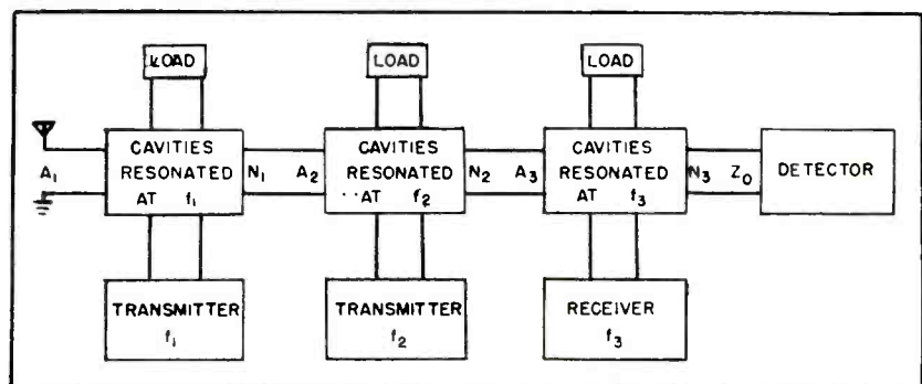
FIG. 8—Arrangement of equipment in three-coupler system. Detector is used for alignment of couplers
