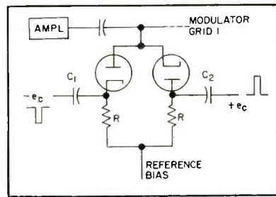
FIG. 9—Synchronous-clamp circuit
