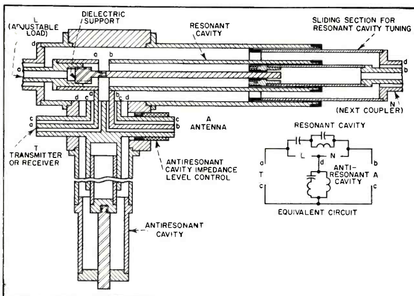
FIG. 5—Cross-section of uhf multicoupler. Letters on diagram refer to points on equivalent circuit
