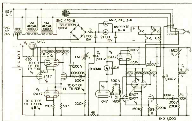
FIG. 4—Complete circuit of preregulator, regulator and d-c filament supply. Adjust rectifier input for hot spot on regulator tubes. The 12AX7 was selected as first amplifier tube in regulator because of its comparatively low noise output. Dry-cell batteries serve as voltage references. Use of d-c heater supply eliminates 60-cps signal modulation
