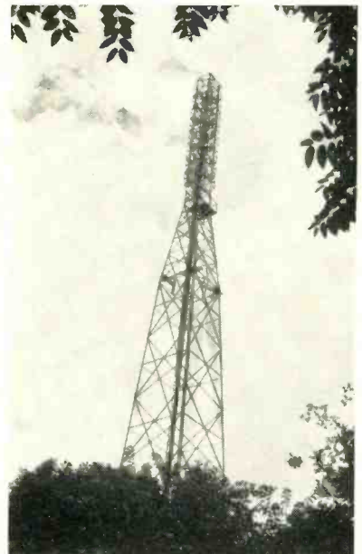
Eight-stack aerial array atop fabricated tower has gain of about sixfold in power when used by England's first commercial television broadcast station. It is located at Croydon and was built for Independent Television Authority by Marconi
