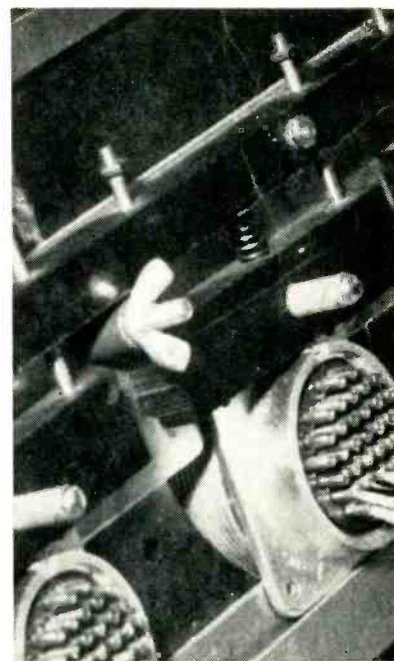
Details of holding fixture. Wing nut can be loosened to slide under strip up or down to accommodate different sizes
