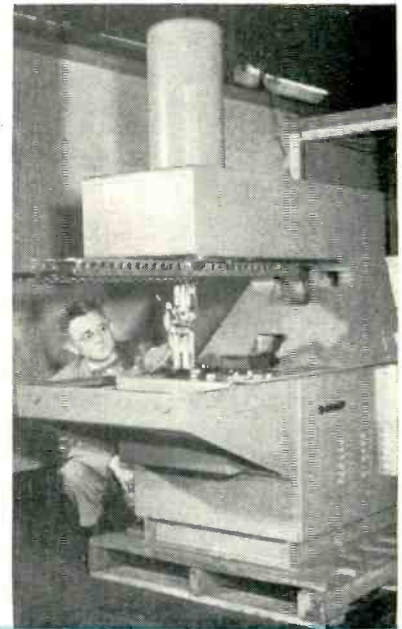
ASSEMBLY MACHINE —Servo-positioned insertion head (right) fits into center of elevator and conveyor mechanism that recycles 20 wiring boards under head until all required components have been inserted one by one. Elevators also provide required storage space at each end to accommodate adjacent machines having different operating times.
