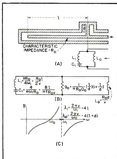
FIG. 4—Physical configuration of antiresonant leg of bridge (A) with equivalent circuit (B) and diagram of susceptance plotted against frequency (C)
